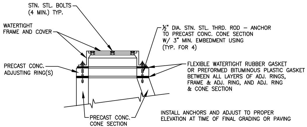
WATERTIGHT FRAME & COVER DETAIL NO SCALE
