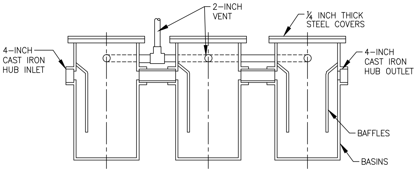
TRIPLE GARAGE BASIN DETAIL DOWNERS GROVE SANITARY DISTRICT
